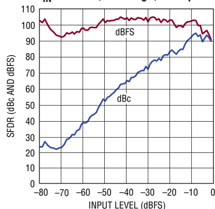
LTC2264-12: SFDR vs Input Level, f_{IN} = 70\text{MHz} , 2\text{V} Range, 40\text{Mpsps}
